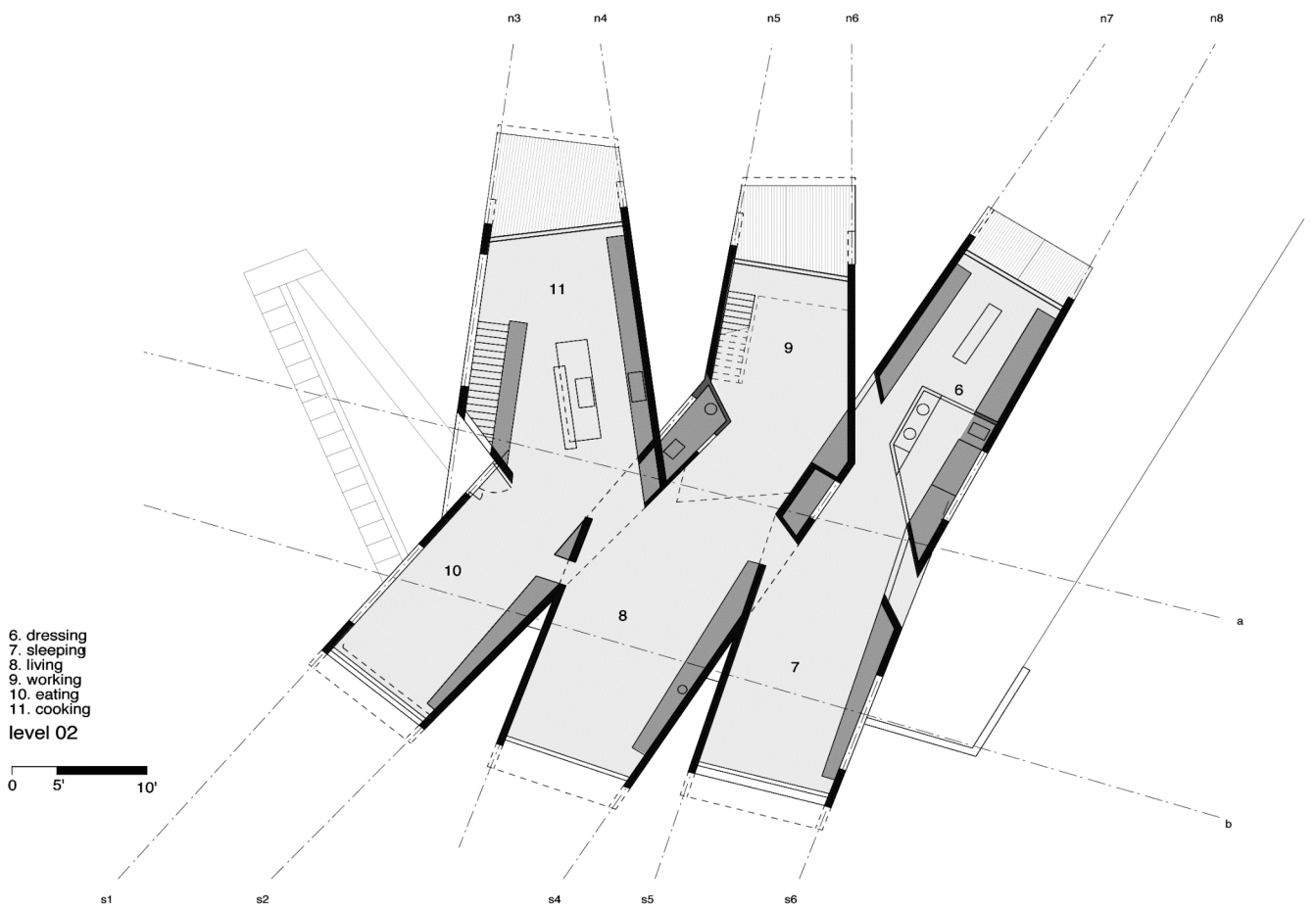
Level 02
