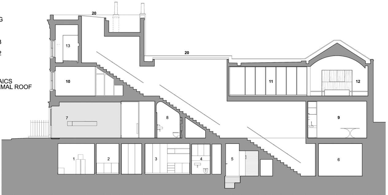
01 SECTION THROUGH LONG STAIRS 1:100
