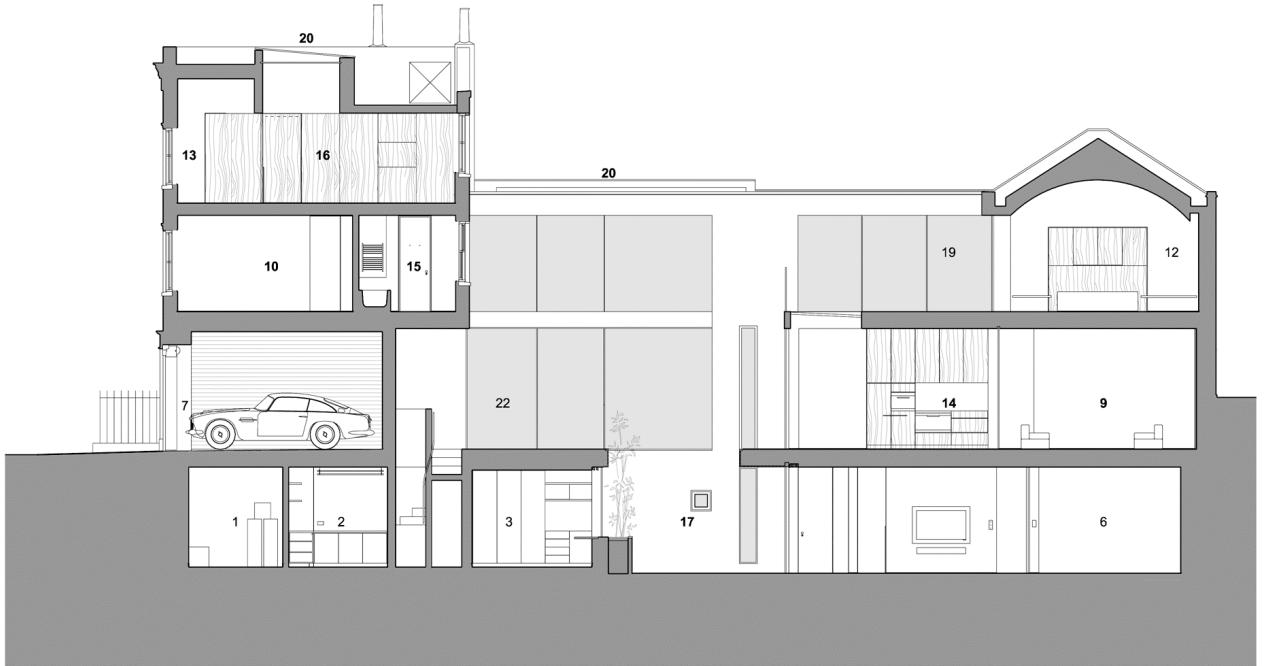
02 SECTION THROUGH COURTYARD 1:100
